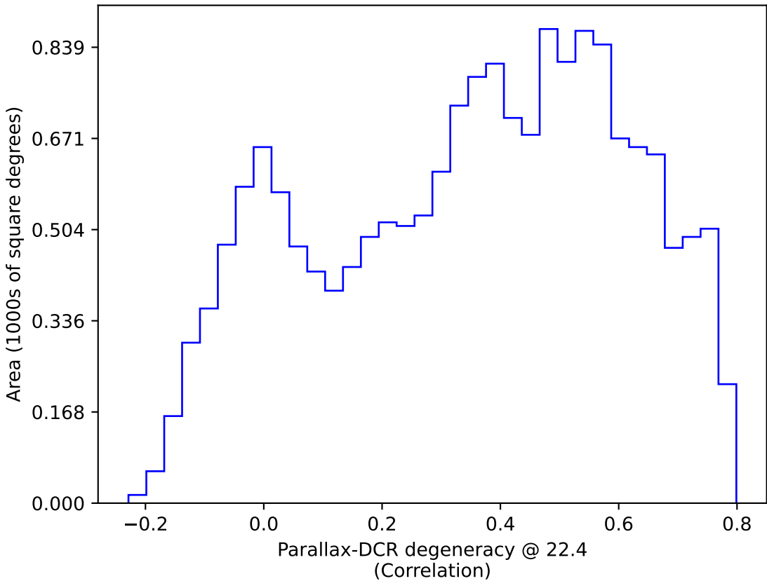
scp_reweight_v3.3_10yrs WFD: Parallax-DCR degeneracy @ 22.4
