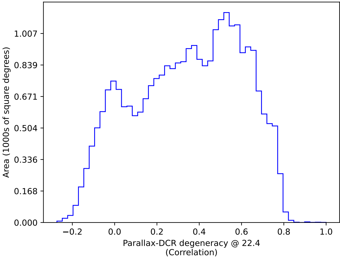
scp_reweight_v3.3_10yrs All sky: Parallax-DCR degeneracy @ 22.4
