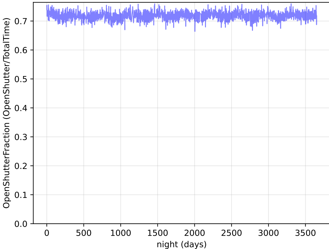
scp_reweight_v3.3_10yrs Per night: OpenShutterFraction
