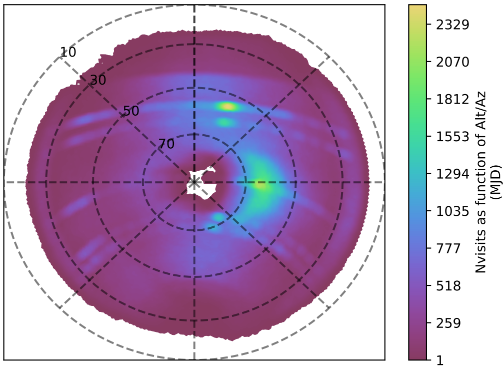
scp_reweight_v3.3_10yrs z band: Nvisits as function of Alt/Az
