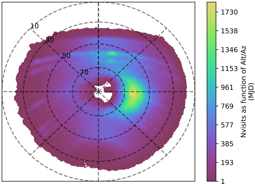
scp_reweight_v3.3_10yrs y band: Nvisits as function of Alt/Az
