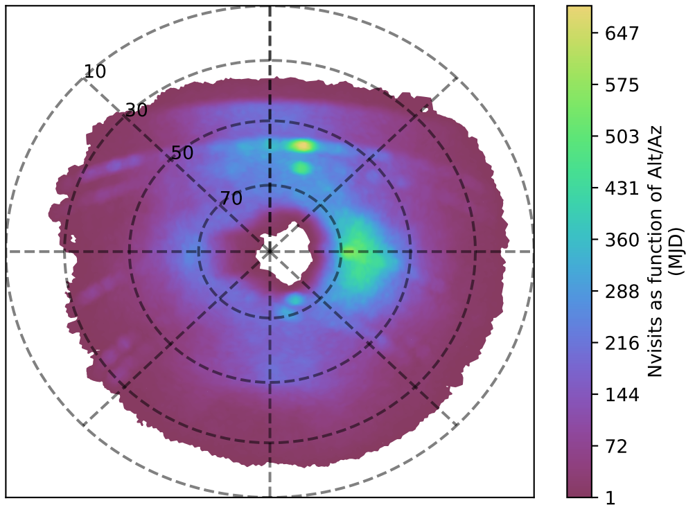
scp_reweight_v3.3_10yrs u band: Nvisits as function of Alt/Az
