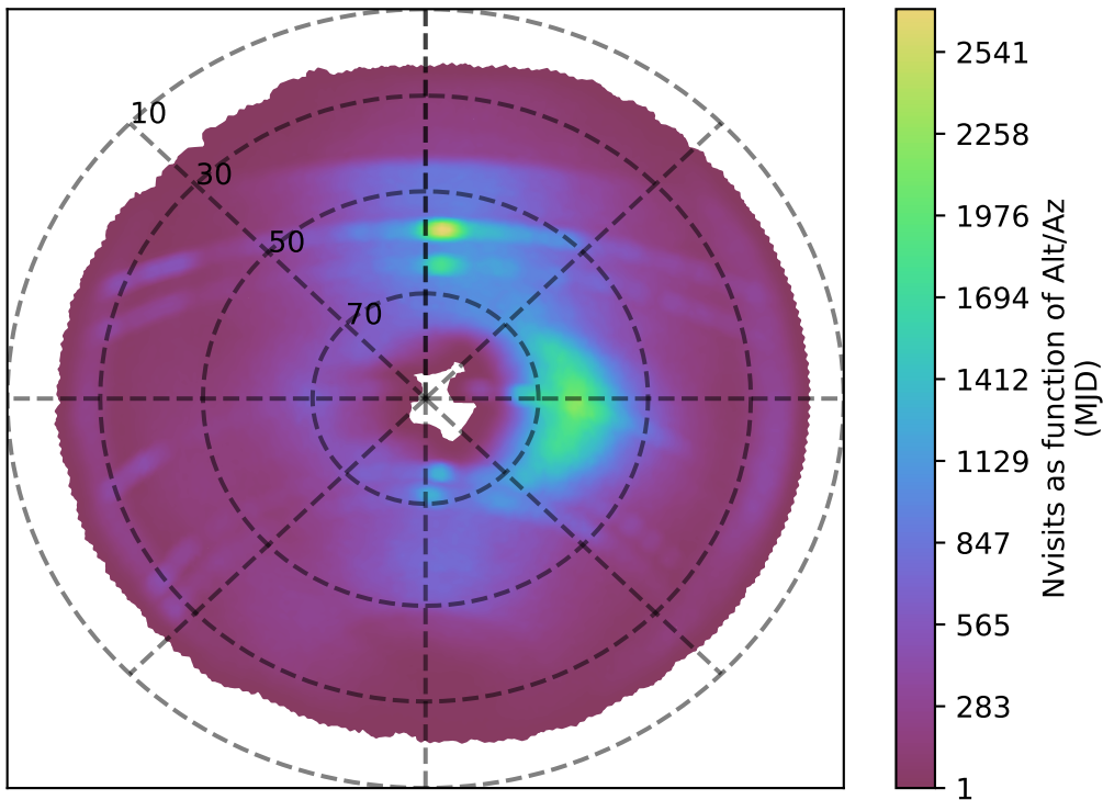
scp_reweight_v3.3_10yrs i band: Nvisits as function of Alt/Az
