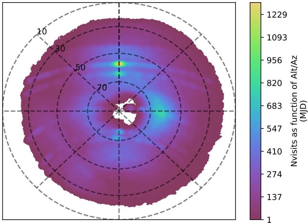
scp_reweight_v3.3_10yrs g band: Nvisits as function of Alt/Az
