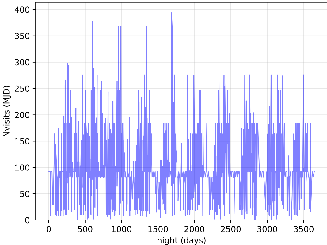
scp_reweight_v3.3_10yrs DDF: Nvisits
