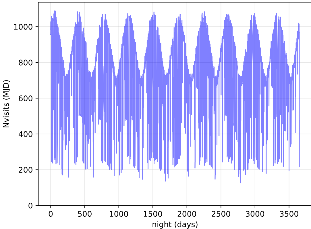
scp_reweight_v3.3_10yrs All visits: Nvisits
