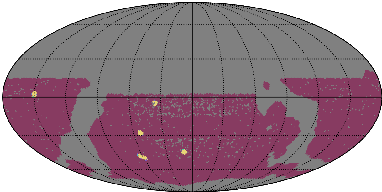
scp_reweight_v3.3_10yrs WFD: NumberOfQuickRevisits
