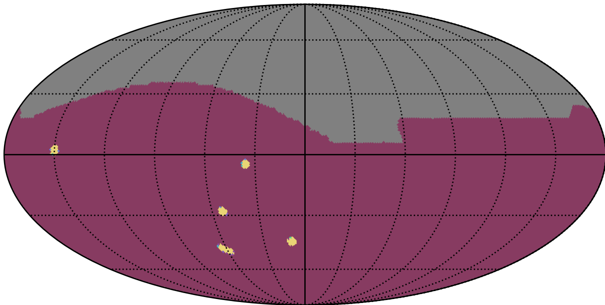
scp_reweight_v3.3_10yrs All sky: NumberOfQuickRevisits
