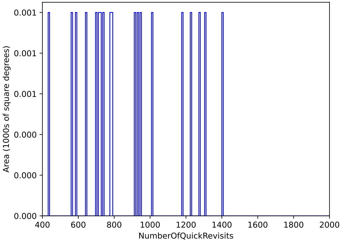
scp_reweight_v3.3_10yrs All sky: NumberOfQuickRevisits
