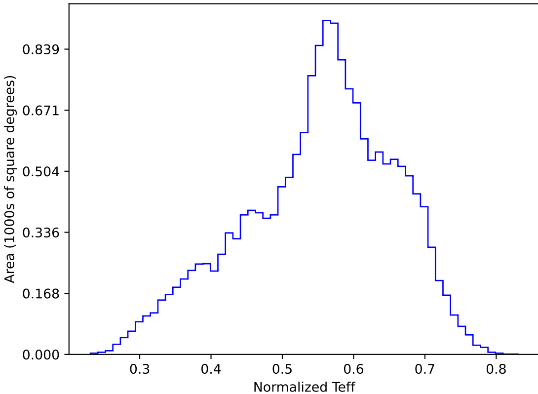
scp_reweight_v3.3_10yrs WFD y band: Normalized Teff
