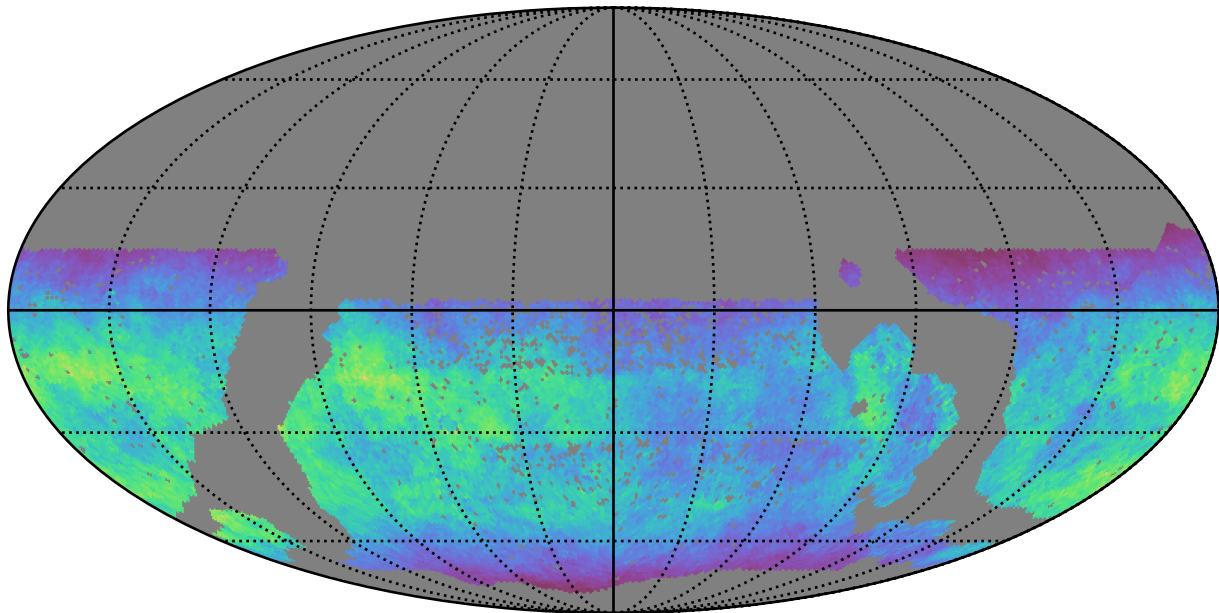
scp_reweight_v3.3_10yrs WFD u band: Normalized Teff
