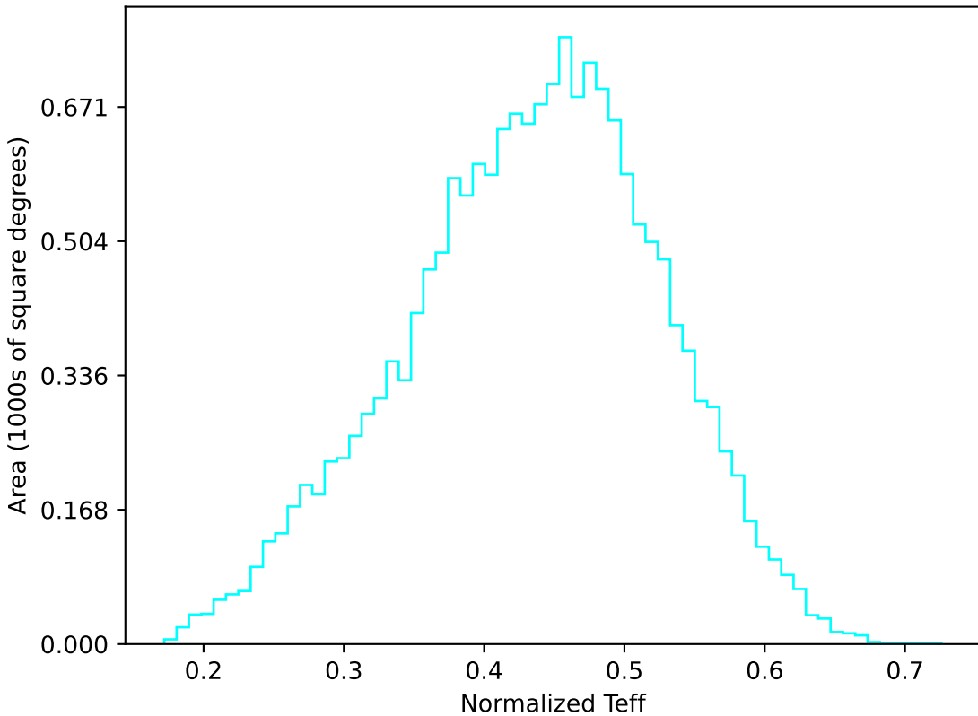
scp_reweight_v3.3_10yrs WFD u band: Normalized Teff
