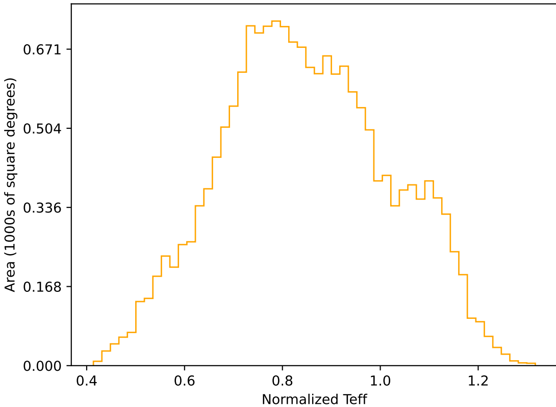
scp_reweight_v3.3_10yrs WFD r band: Normalized Teff
