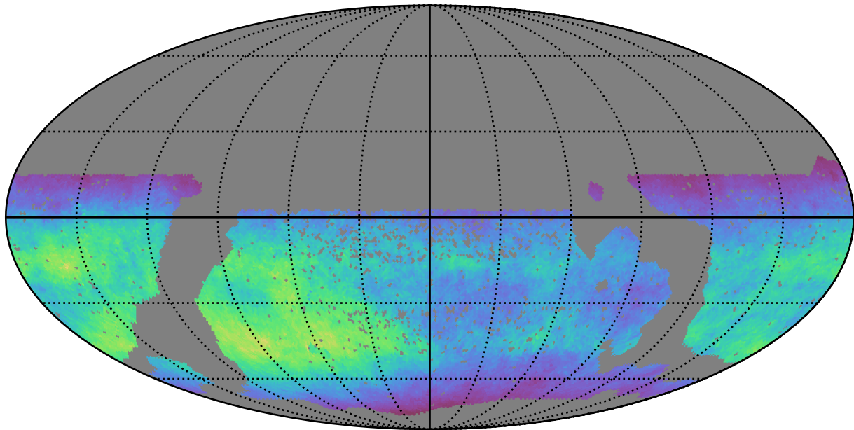
scp_reweight_v3.3_10yrs WFD i band: Normalized Teff
