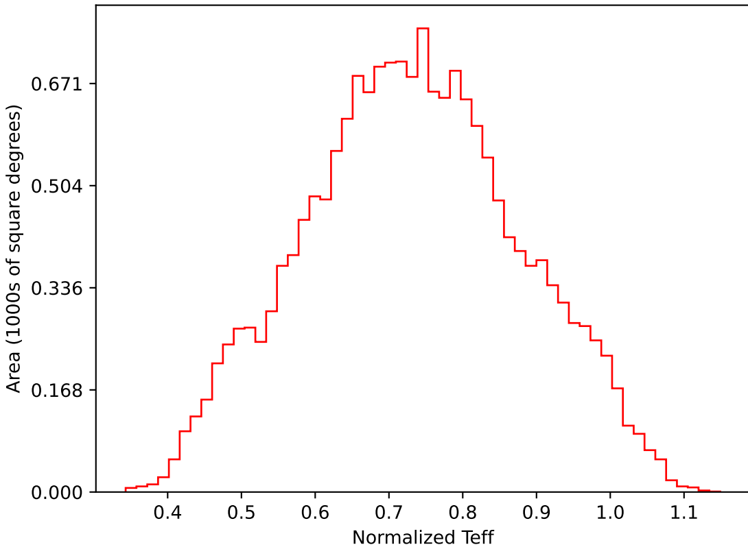
scp_reweight_v3.3_10yrs WFD i band: Normalized Teff
