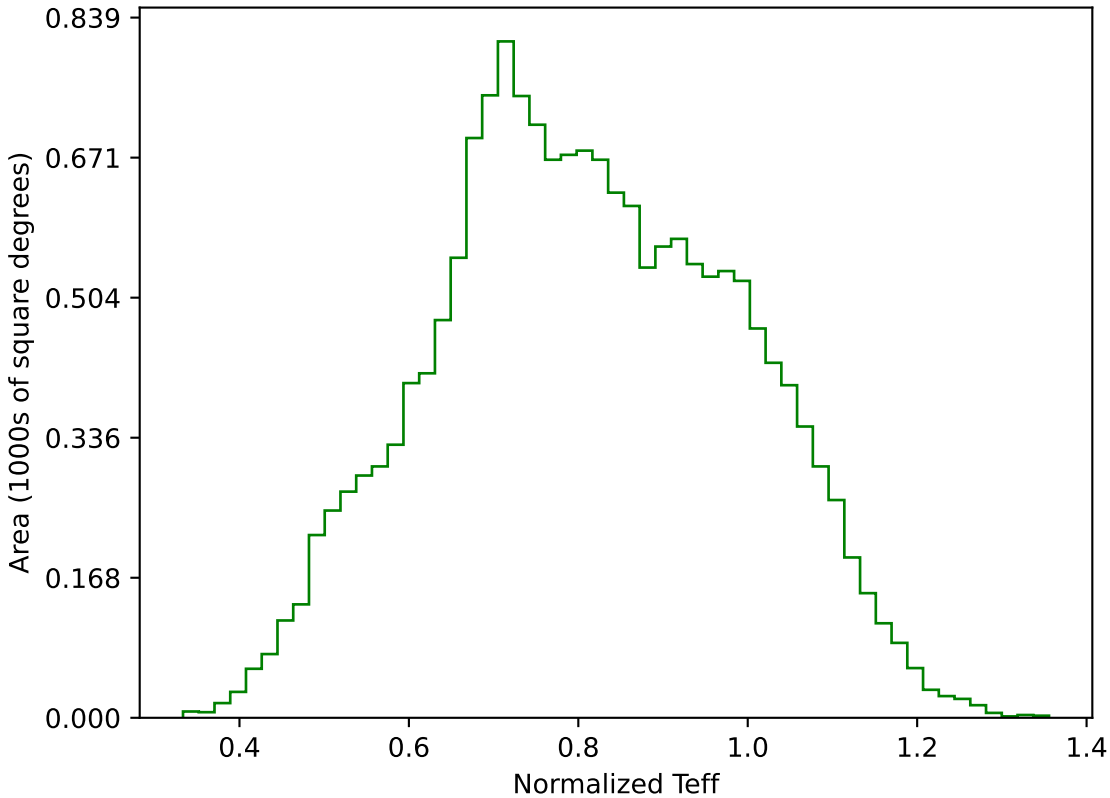
scp_reweight_v3.3_10yrs WFD g band: Normalized Teff
