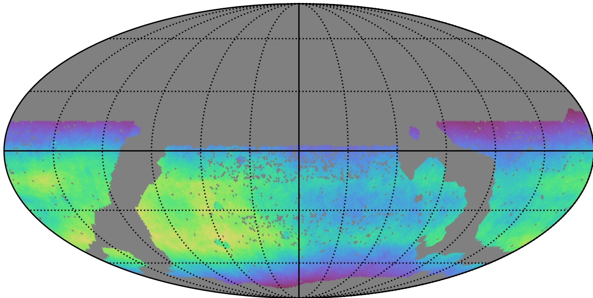
scp_reweight_v3.3_10yrs WFD all bands: Normalized Teff
