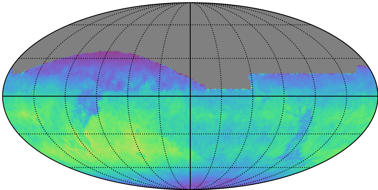
scp_reweight_v3.3_10yrs All sky z band: Normalized Teff
