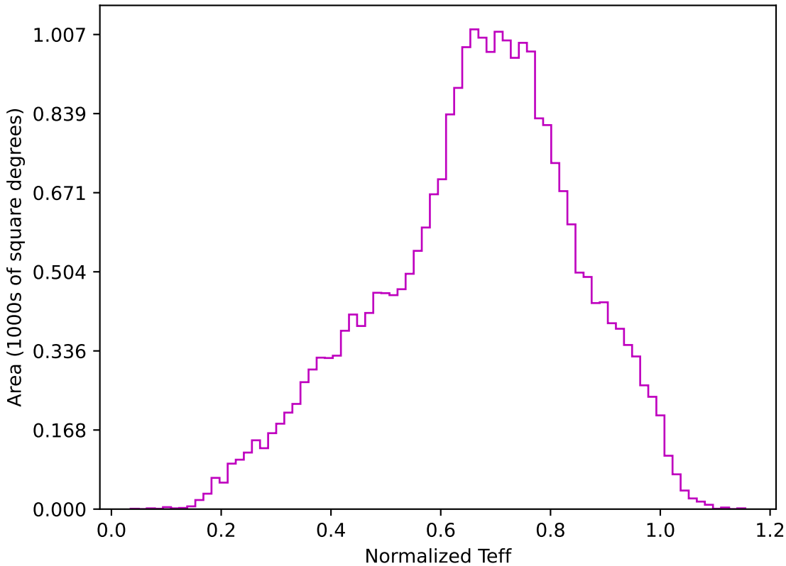
scp_reweight_v3.3_10yrs All sky z band: Normalized Teff
