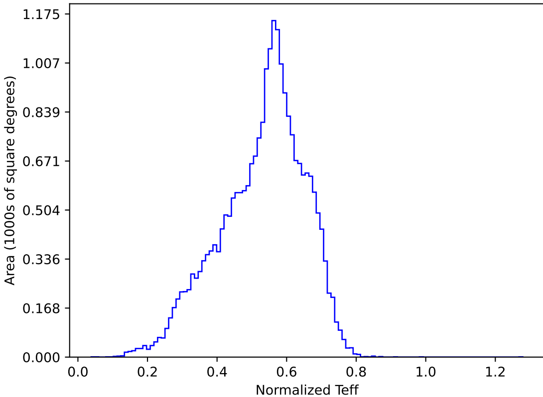
scp_reweight_v3.3_10yrs All sky y band: Normalized Teff
