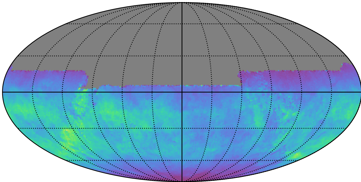
scp_reweight_v3.3_10yrs All sky u band: Normalized Teff
