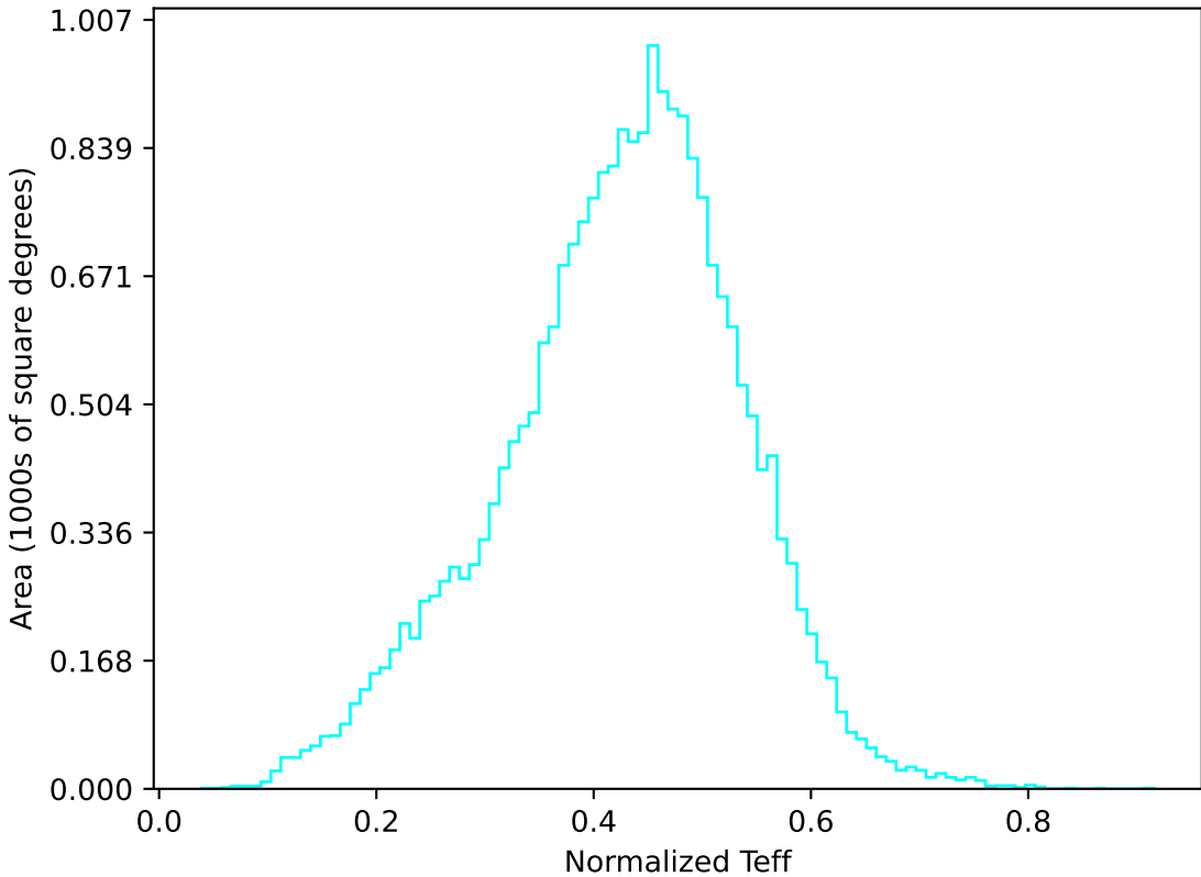
scp_reweight_v3.3_10yrs All sky u band: Normalized Teff
