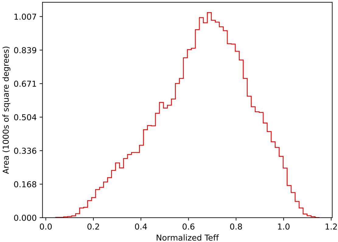
scp_reweight_v3.3_10yrs All sky i band: Normalized Teff
