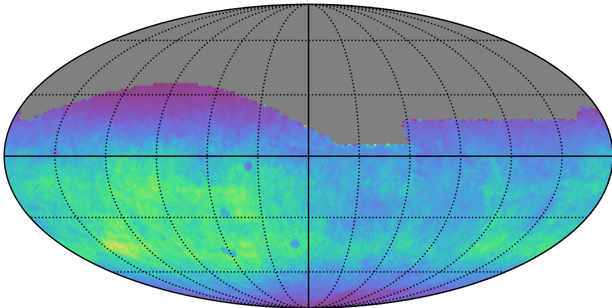
scp_reweight_v3.3_10yrs All sky g band: Normalized Teff
