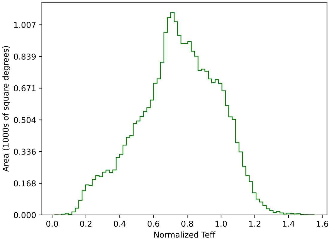
scp_reweight_v3.3_10yrs All sky g band: Normalized Teff
