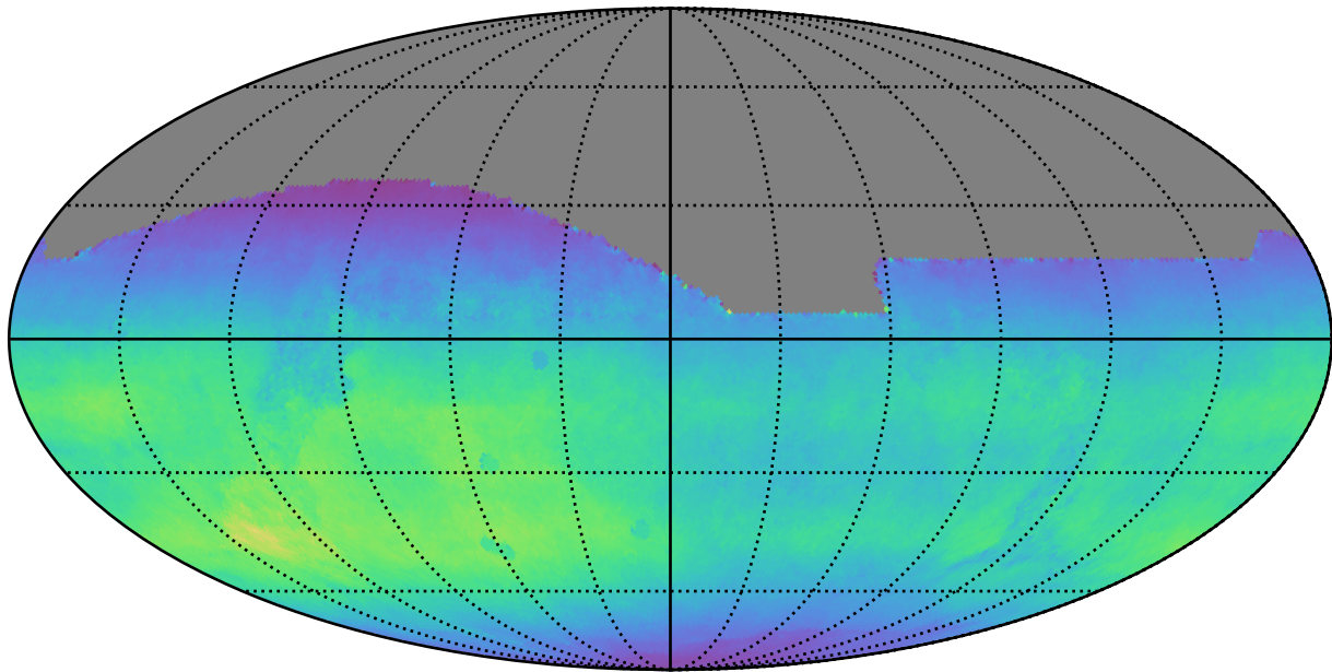
scp_reweight_v3.3_10yrs All sky all bands: Normalized Teff
