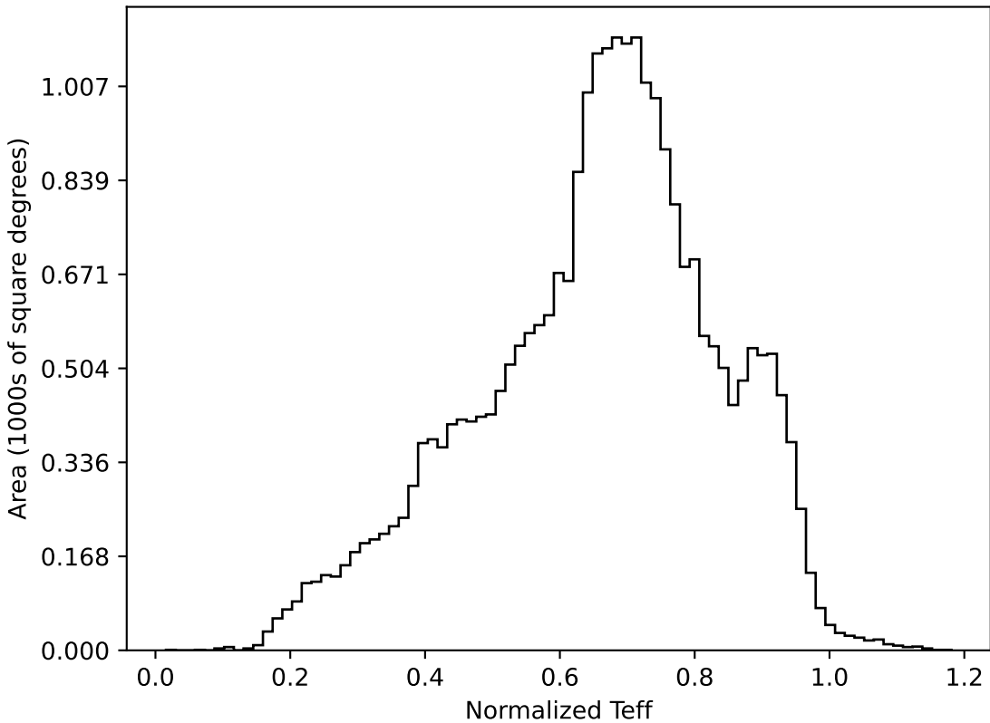
scp_reweight_v3.3_10yrs All sky all bands: Normalized Teff
