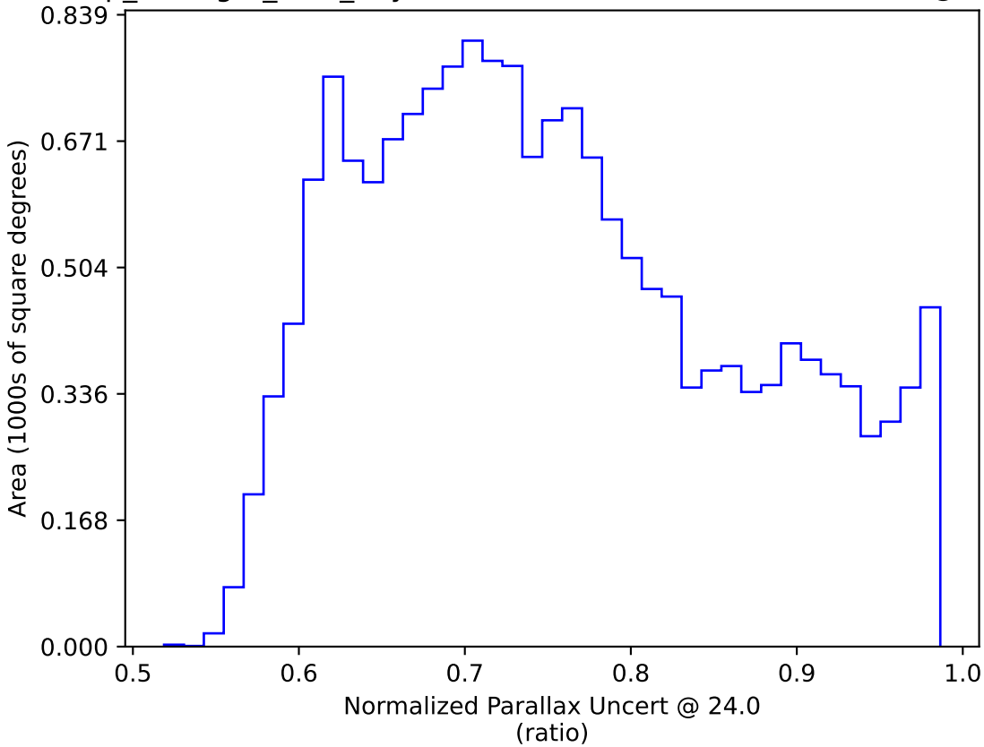
scp_reweight_v3.3_10yrs WFD: Normalized Parallax Uncert @ 24.0
