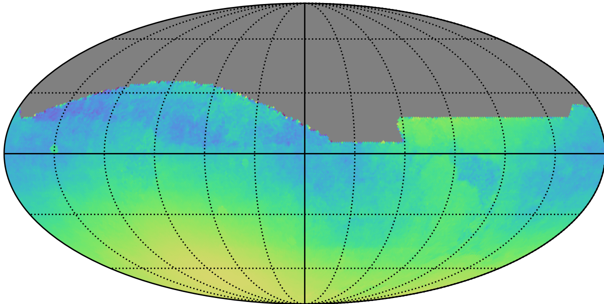
scp_reweight_v3.3_10yrs All sky: Normalized Parallax Uncert @ 24.0
