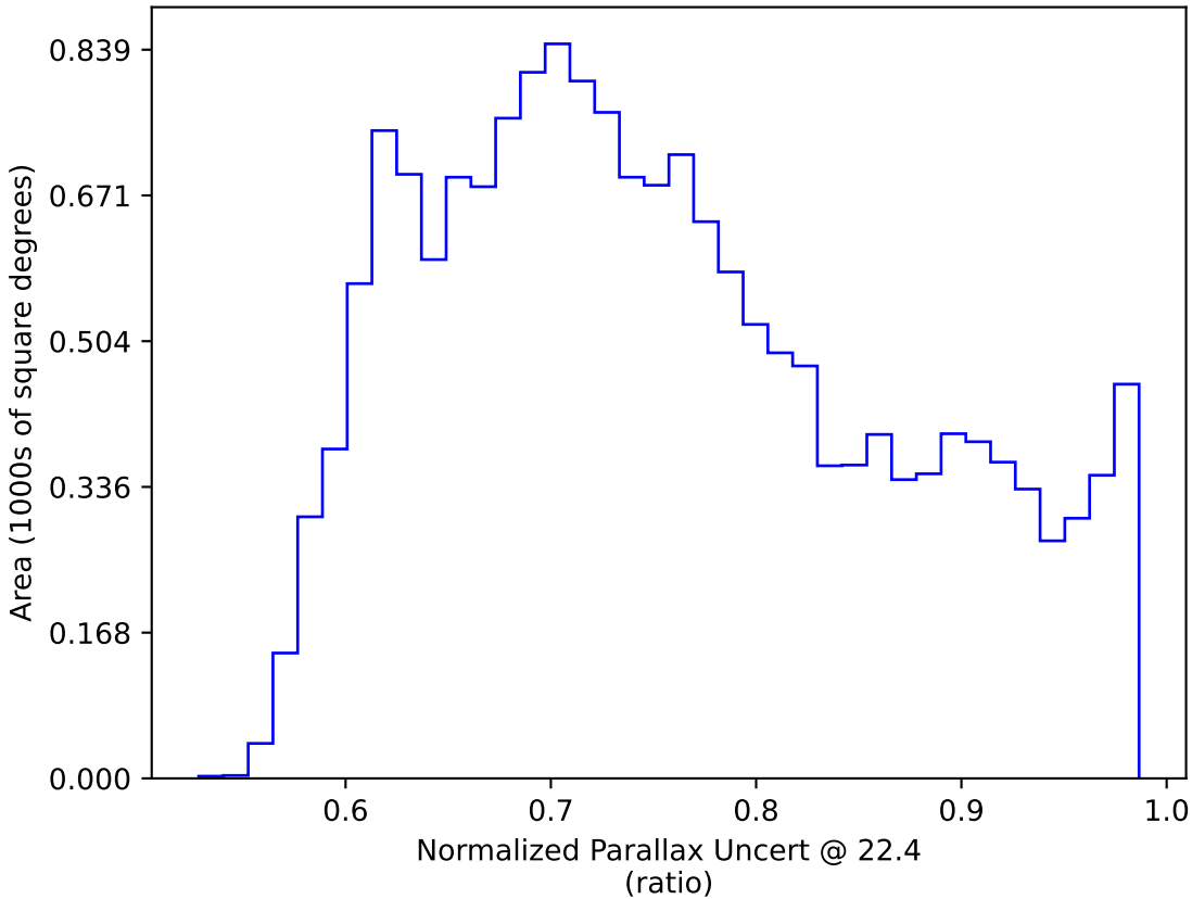
scp_reweight_v3.3_10yrs WFD: Normalized Parallax Uncert @ 22.4
