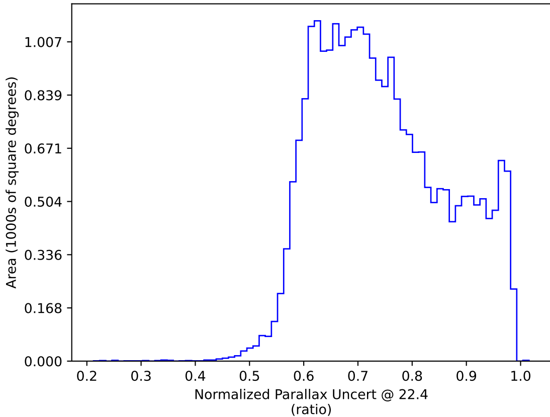
scp_reweight_v3.3_10yrs All sky: Normalized Parallax Uncert @ 22.4
