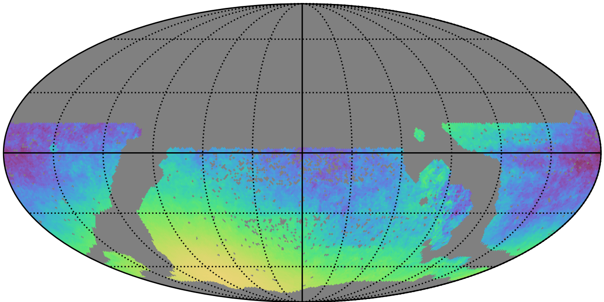
scp_reweight_v3.3_10yrs WFD y band only: Normalized Parallax Uncert @ 21.3
