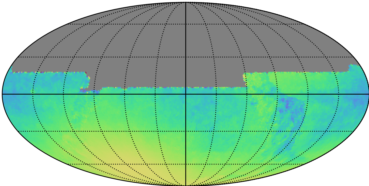
scp_reweight_v3.3_10yrs All sky y band only: Normalized Parallax Uncert @ 21.3
