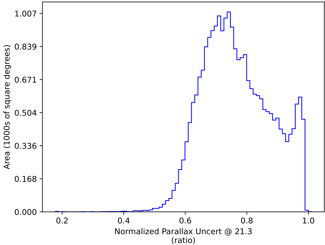
scp_reweight_v3.3_10yrs All sky y band only: Normalized Parallax Uncert @ 21.3
