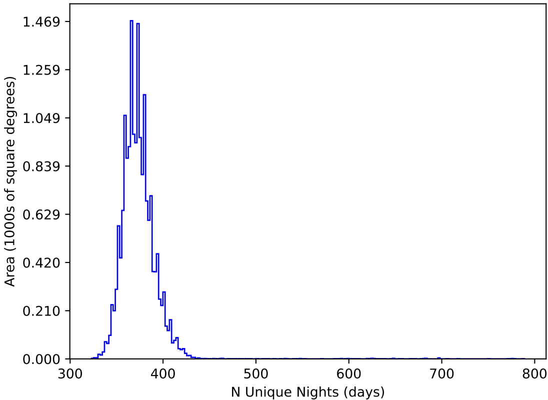
scp_reweight_v3.3_10yrs WFD all bands: N Unique Nights
