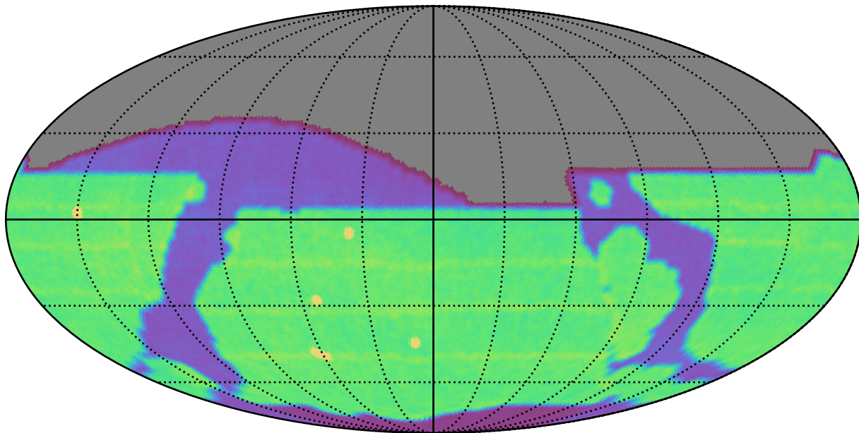
scp_reweight_v3.3_10yrs All sky all bands: N Unique Nights
