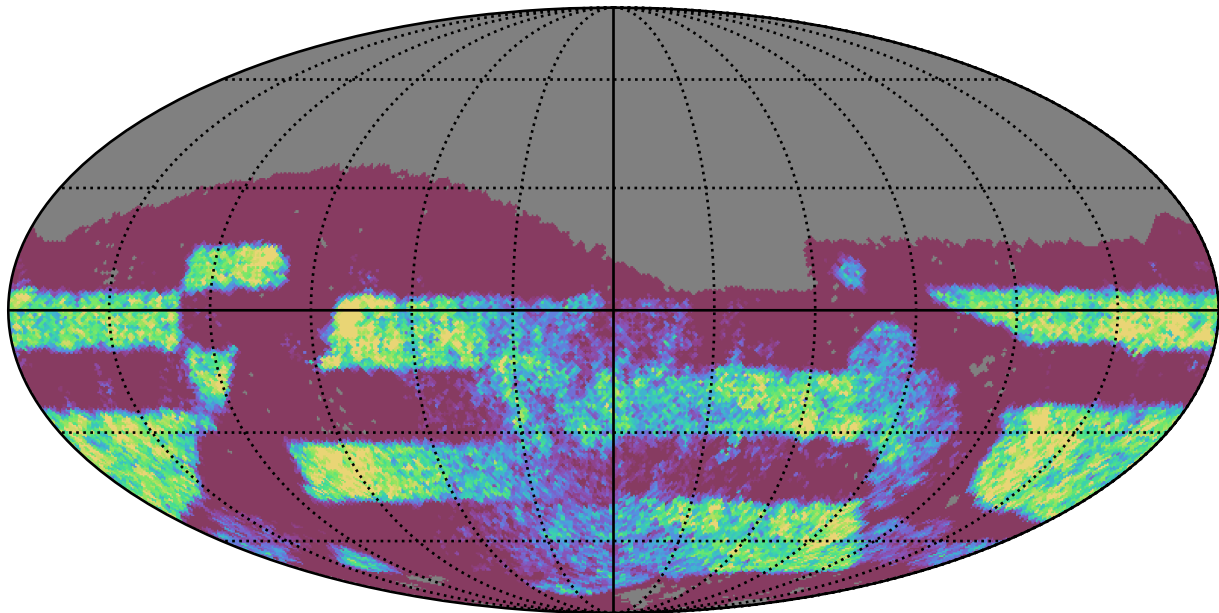
scp_reweight_v3.3_10yrs Yr 3-4 z band: NVisits
