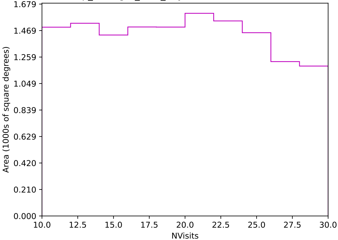
scp_reweight_v3.3_10yrs Yr 3-4 z band: NVisits
