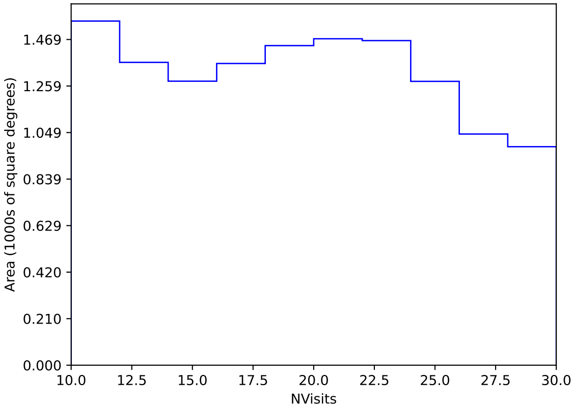
scp_reweight_v3.3_10yrs Yr 3-4 y band: NVisits
