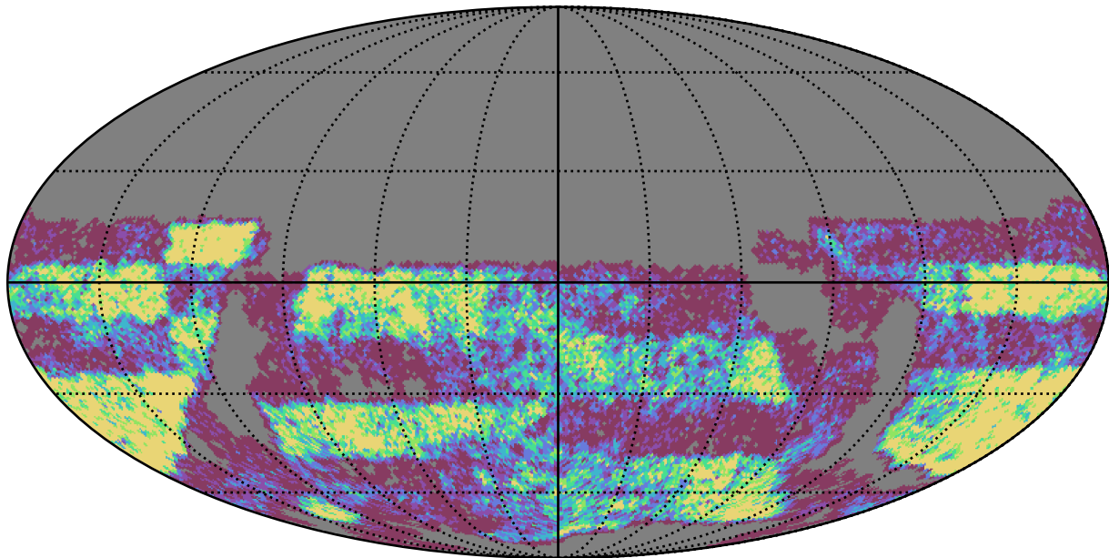
scp_reweight_v3.3_10yrs Yr 3-4 u band: NVisits
