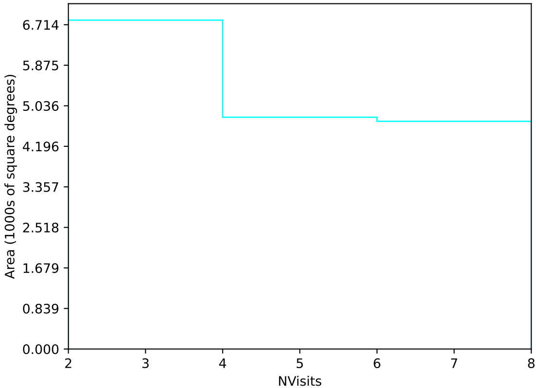
scp_reweight_v3.3_10yrs Yr 3-4 u band: NVisits
