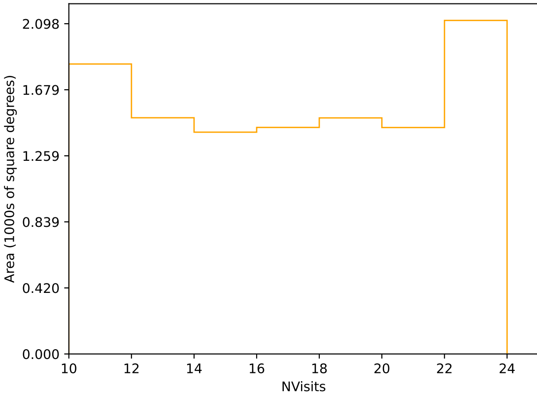
scp_reweight_v3.3_10yrs Yr 3-4 r band: NVisits
