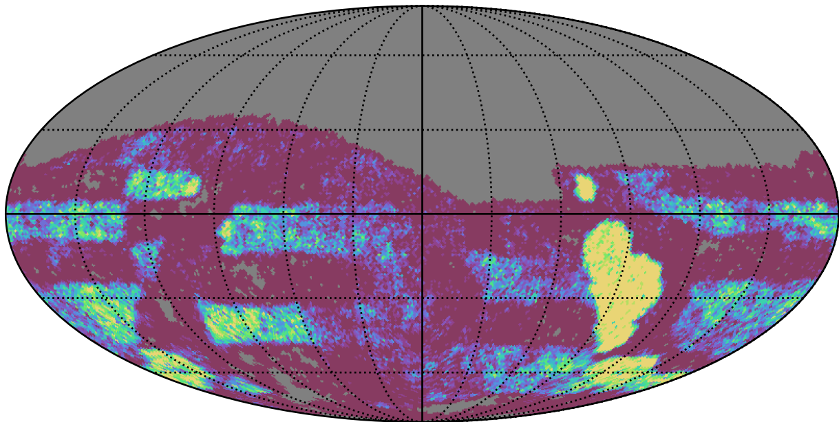
scp_reweight_v3.3_10yrs Yr 3-4 g band: NVisits
