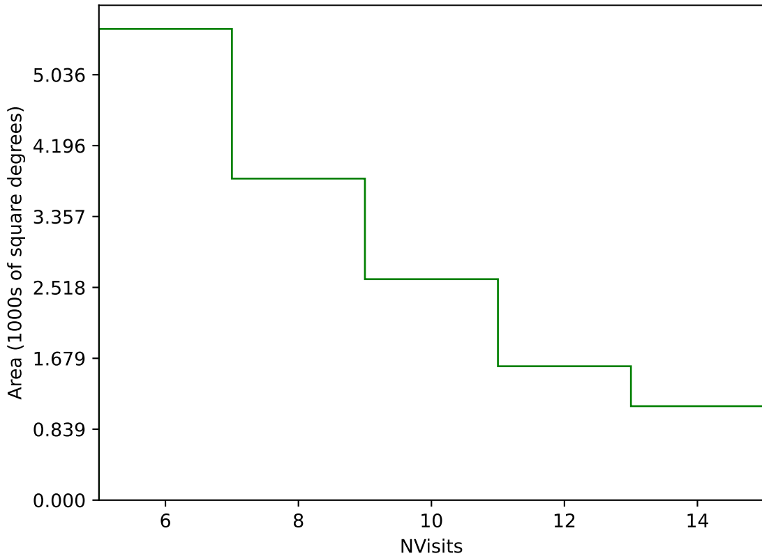
scp_reweight_v3.3_10yrs Yr 3-4 g band: NVisits
