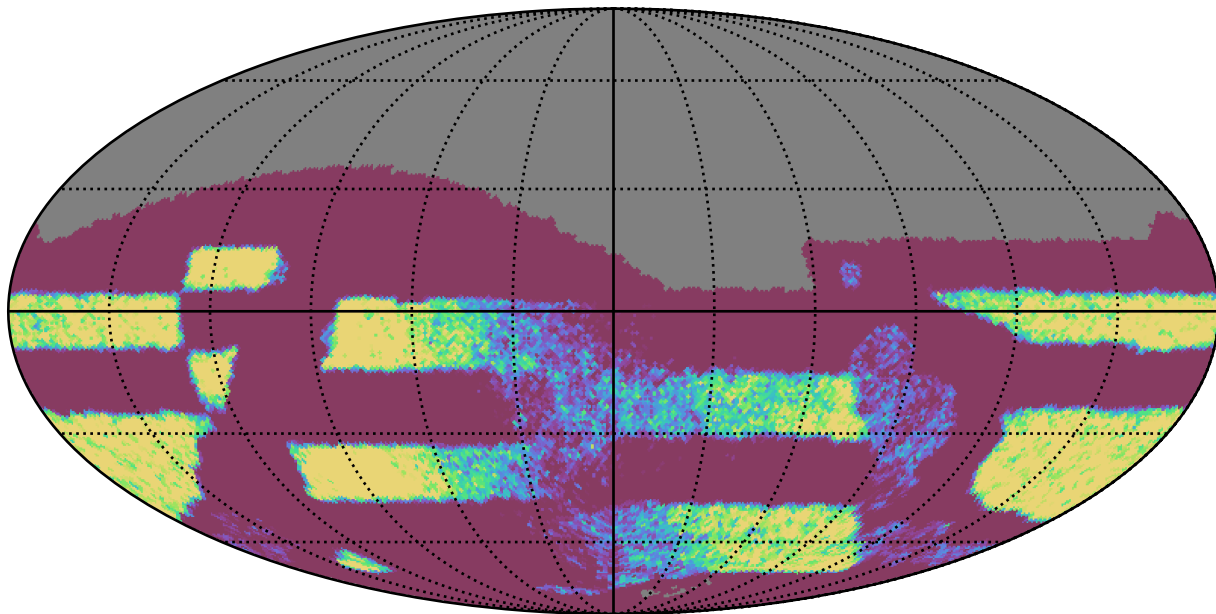
scp_reweight_v3.3_10yrs Yr 3-4 all bands: NVisits
