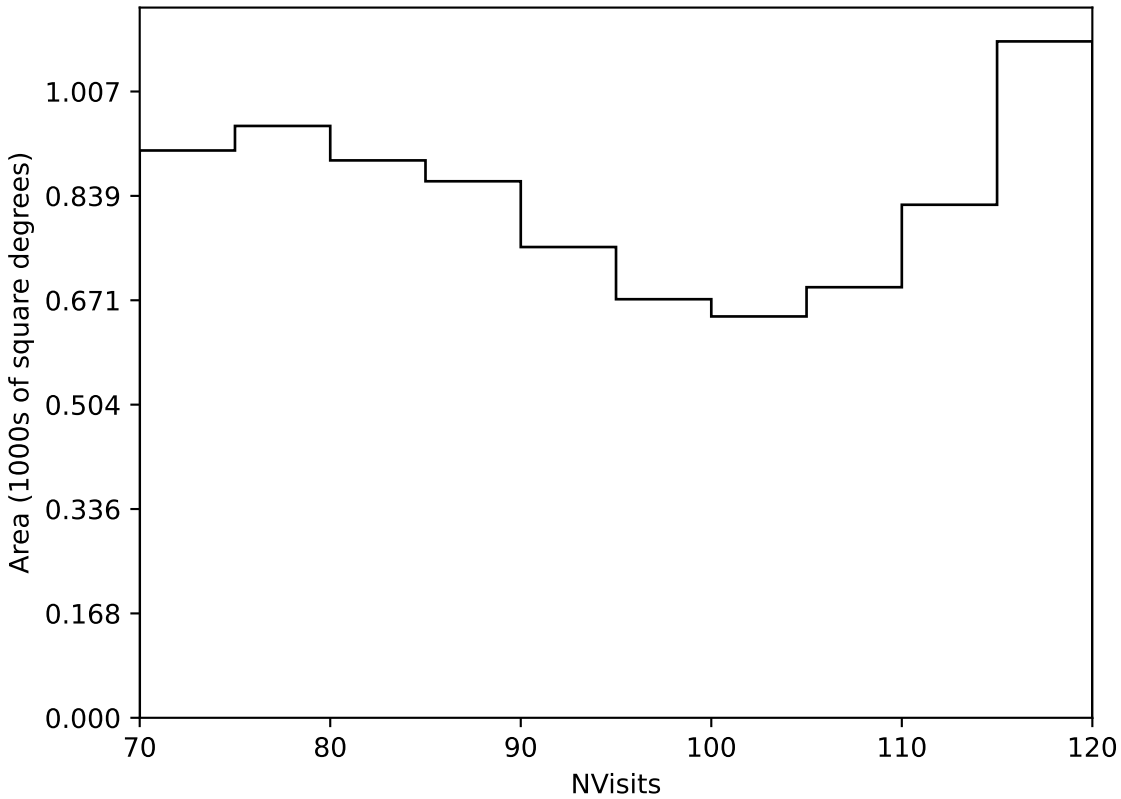
scp_reweight_v3.3_10yrs Yr 3-4 all bands: NVisits
